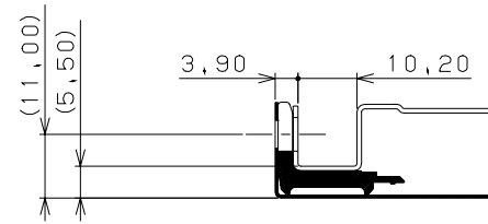
Detail I' -I'
