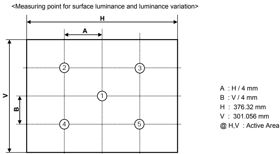
Figure 6. Luminance measuring point
